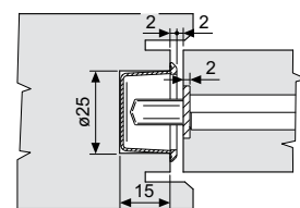
Drilling for the covering tray for Scivola T
