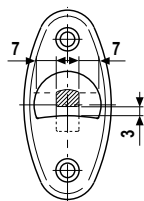
HOOK DETAIL
